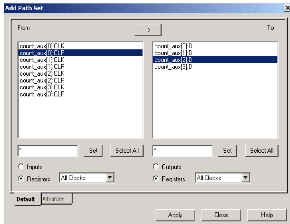
Add Path Set Dialog Box
